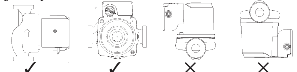
Fig 5 Pump Installation Positions
