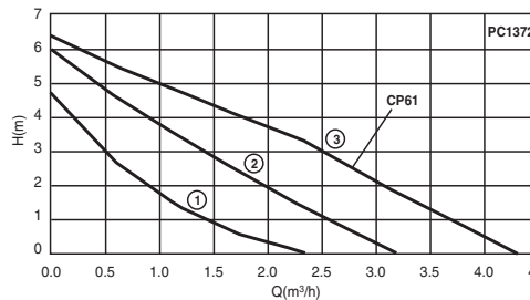
Fig 4 CP61/63 Performance Curve - 230V ~ 50Hz
