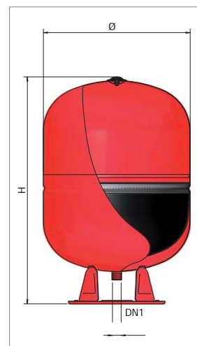
ERCE 80 - 500
