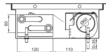
CONVECTOR SECTION
